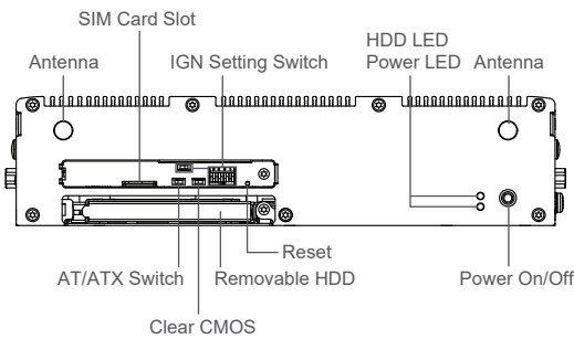
Front I/O
